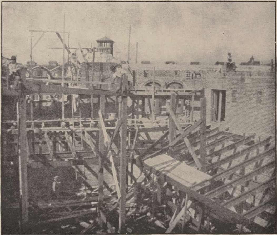
BUILDING THE ROOF STAGING.
